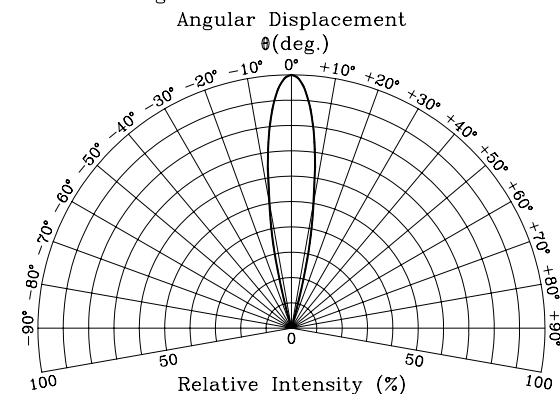
Radiation Diagram
